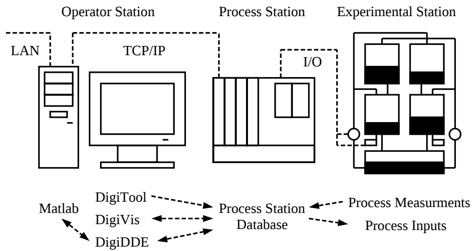
Figure 3: Schematic of the control system
