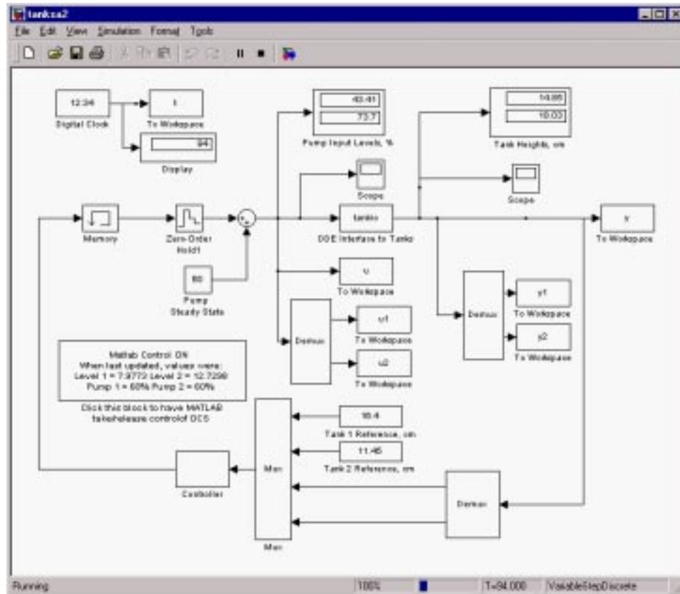
Figure 6: Screenshot of the Matlab Interface
