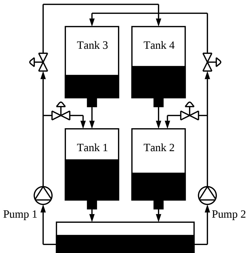
Figure 1: Schematic of the four tank system
