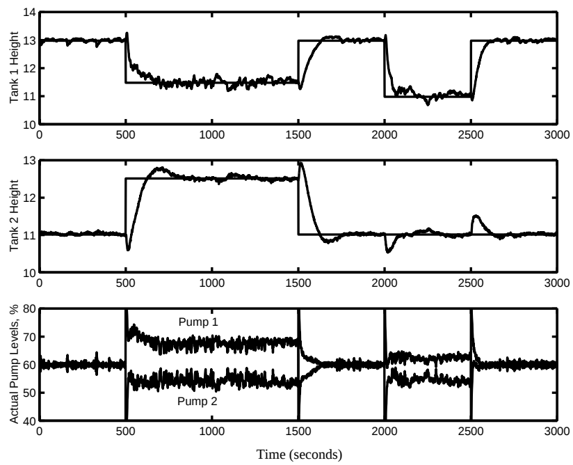
Figure 8: Reference tracking using robust controller
