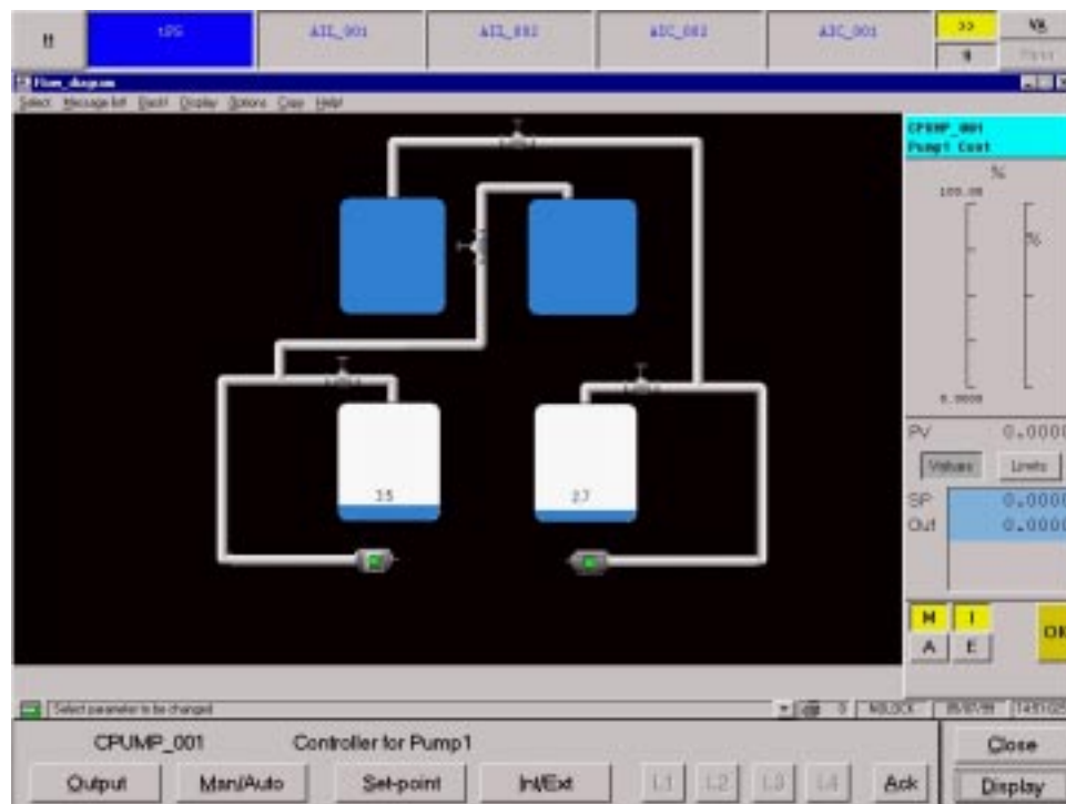
Figure 4: Screenshot of Freelance four tank schematic
