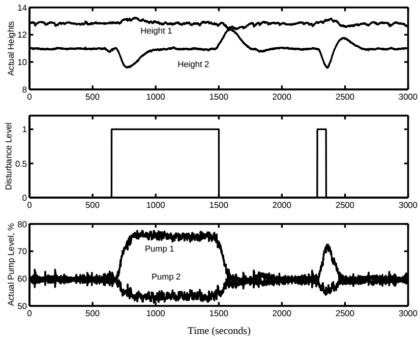
Figure 7: Disturbance rejection using robust controller
