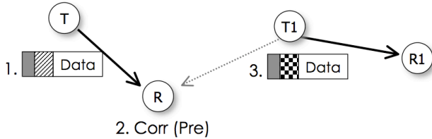
Figure 3: While receiving from T , the receiver R searches for a preamble via correlation (denoted \text{Corr(Pre)} ).
