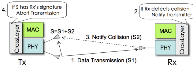
Figure 1: Basic structure of CSMA/CN.
