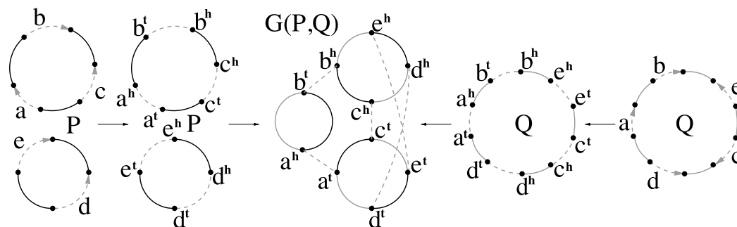
FIG. 1. The breakpoint graph G(P, Q) of a two-chromosomal genome P = (+a + b - c)(-d + e) and a unichromosomal genome Q = (+a + b - e + c - d) represented as two black-obverse cycles and a gray-obverse cycle correspondingly.
