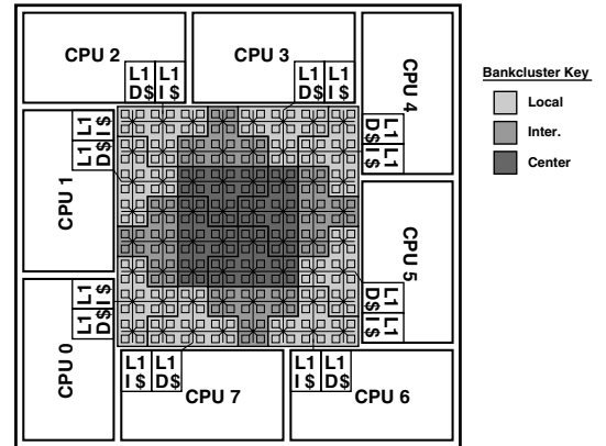
Figure 1. CMP-SNUCA Layout with CMP-DNUCA Bankcluster Regions
