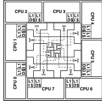
Figure 3. CMP-Hybrid Layout
