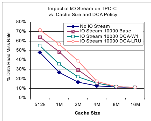
Figure 8. Impact of Limiting I/O Stream Allocation to a Single Way (8-way caches assumed)
