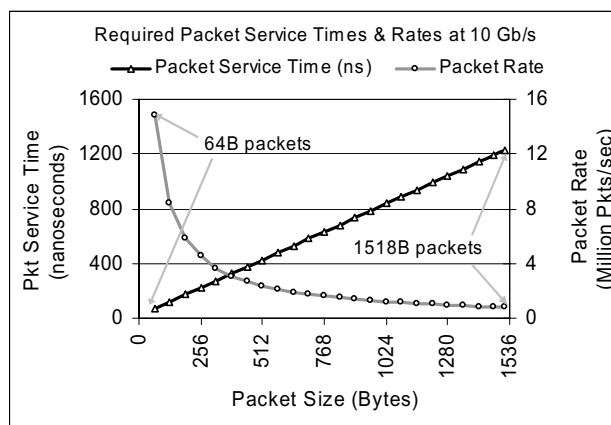
Figure 1. Expected Packet Service Time and Packet Rates at 10 Gb/s versus Packet Size
