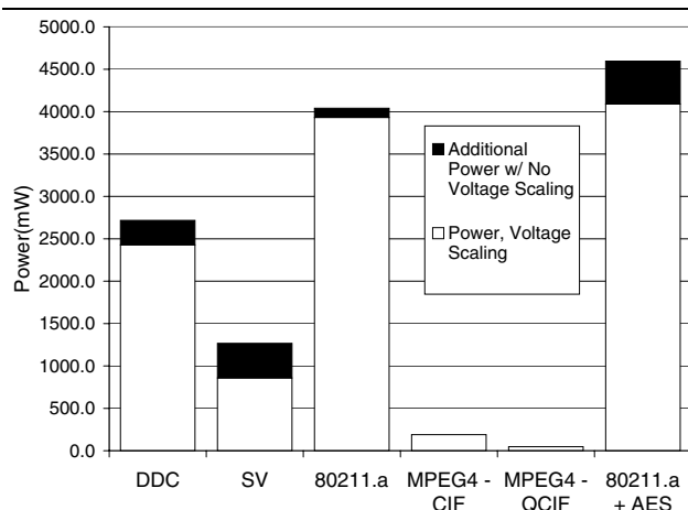
Figure 6. Power Consumption by Application
