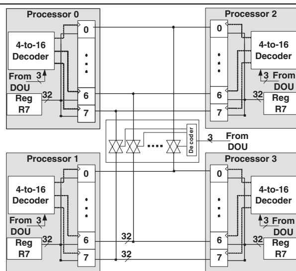
Figure 2. Segment Controllers
