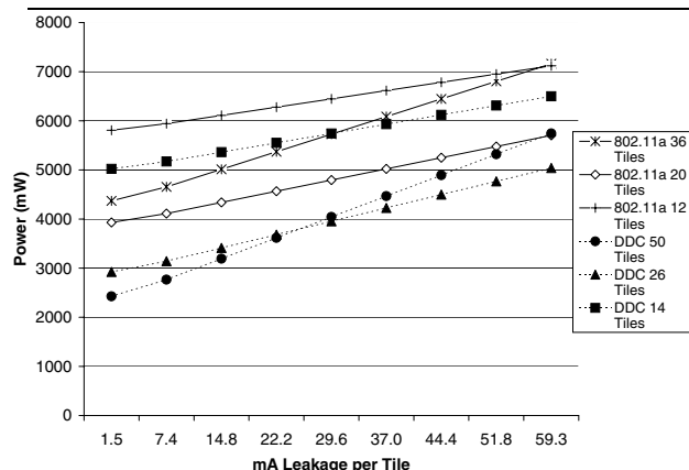
Figure 9. Leakage sensitivity for DDC, 802.11a
