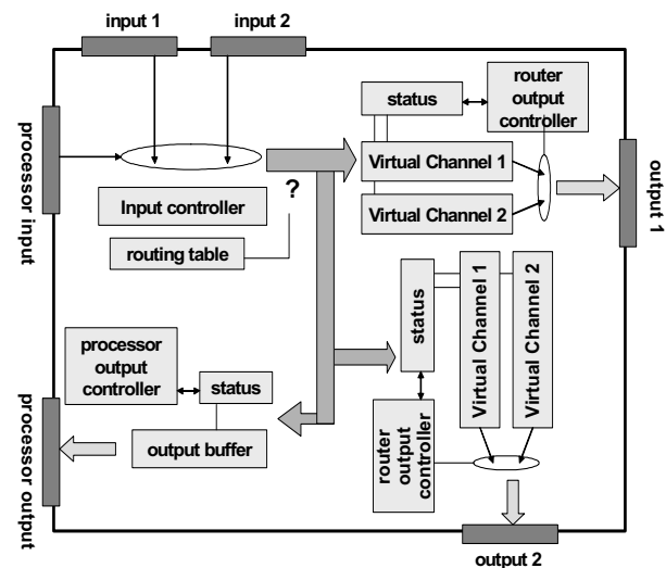
Figure 3: 2D Router's architecture
