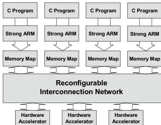
Figure 5: System Simulation Platform
