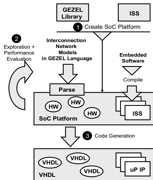
Figure 1: GEZEL System Exploration and Code Generation Process
