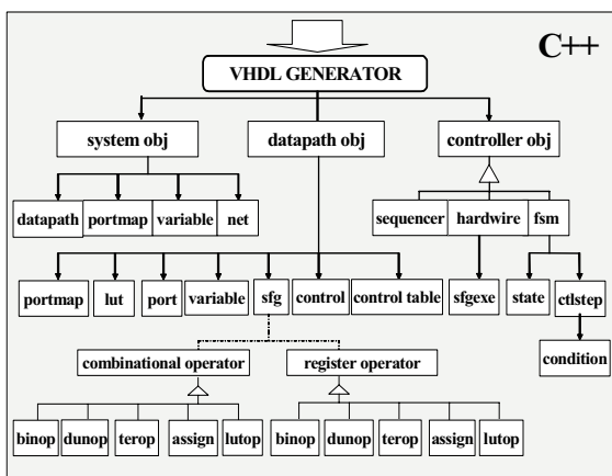
Figure 7: Code Generator object structure
