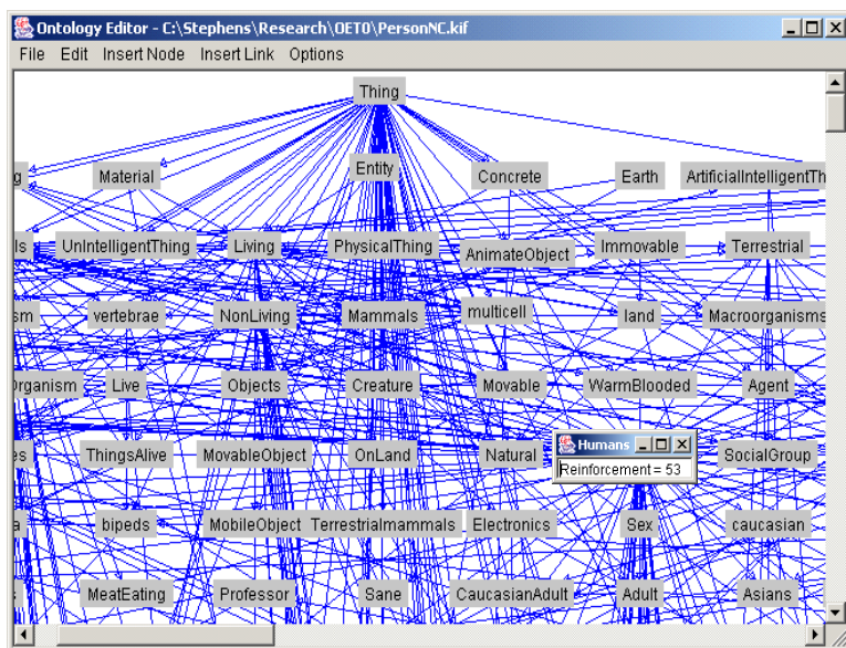
Figure 2: A portion of the ontology formed by merging 54 independently constructed ontologies for the domain Humans/People/Persons. The entire ontology has 389 concepts related by 696 subclass links.
