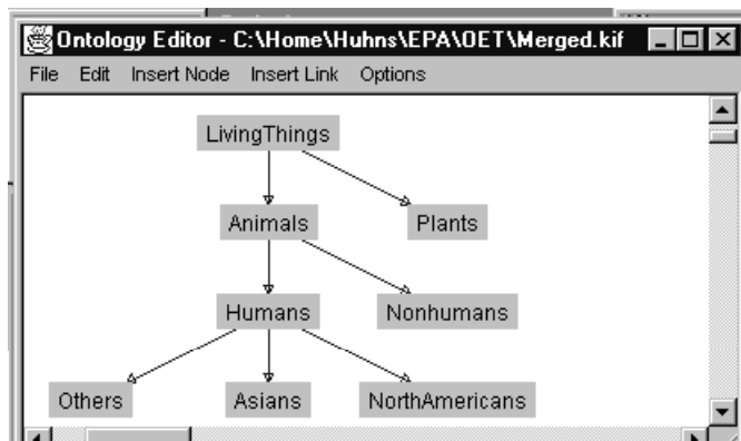
Figure 1: A typical small ontology used to characterize an information source about people (all links denote subclasses)
