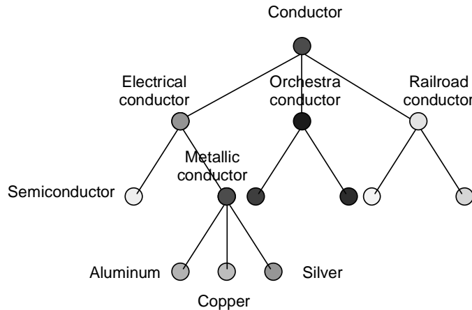
Figure 4: A merged ontology refines the domain concepts needed by users to satisfy their requests.
