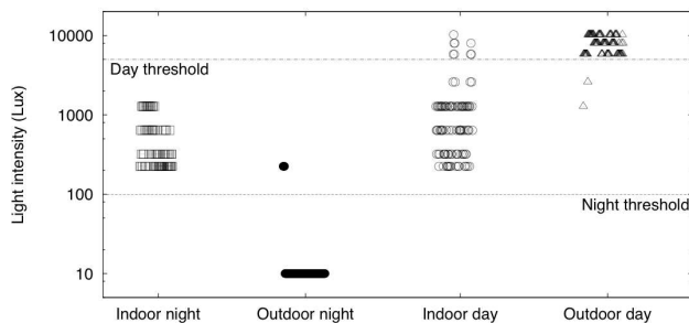
Fig. 7. Indoor/outdoor light intensities
