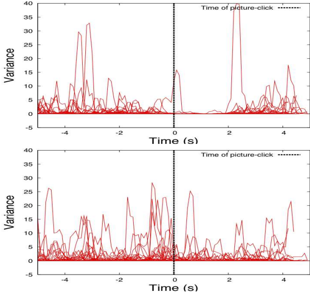
Fig. 3. Variance of accelerometer readings from phones of (a) those in the picture and (b) those outside the picture. Posing signature is evident in (a) and absent in (b).
