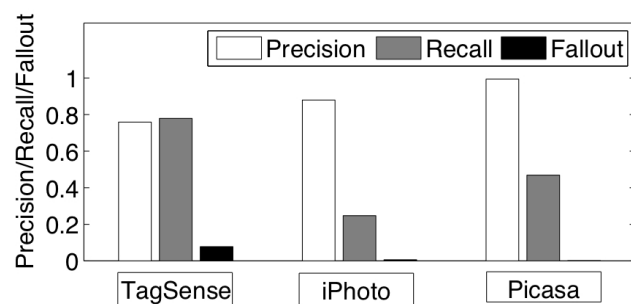
Fig. 11. The overall precision of TagSense is not as high as iPhoto and Picasa, but its recall is much better, while their fall-out is comparable.
