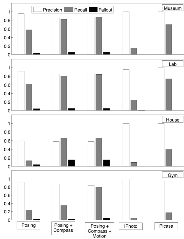
Fig. 12. The performance of different TagSense methods under different scenarios (from top to bottom): (a) museum, (b) lab, (c) house, and (d) gym.
