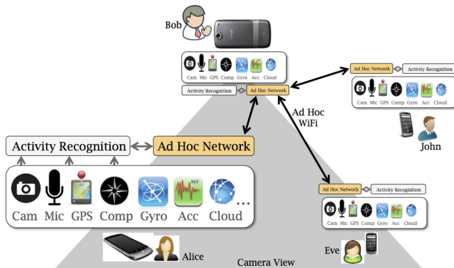
Fig. 2. TagSense architecture – the camera phone triggers sensing in participating phones and gathers the sensed information. It then determines who is in the picture and tags it with the people and the context.
