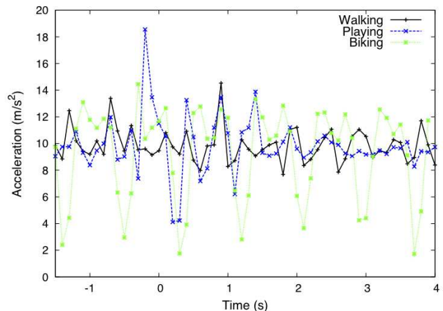
Fig. 6. Acceleration readings for different activities.
