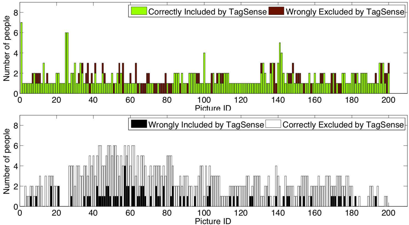
Fig. 8. Performance of TagSense: (a) Top and (b) bottom graphs show people inside and outside each picture. Wrongly excluded/included ones are shown in red/black. Overall, TagSense does well in tagging people.
