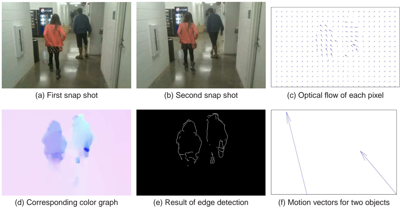
Fig. 5. The illustration of the procedure for extracting motion vectors of people from two successive snapshots.
