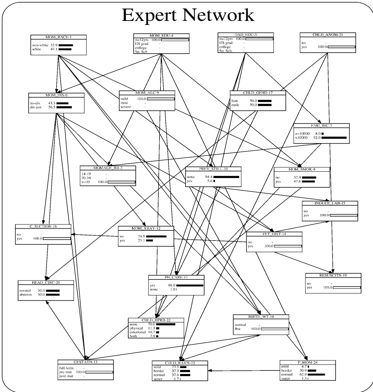
Figure 5: Probabilities in the expert network for a high risk case.
